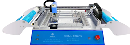
CHM-T36VB (58 feeders, PC control)
